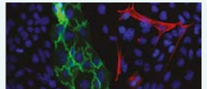
Figure 1: Immunofluorescence staining of PECAM1 (11256-1-AP), Alexa 488 goat anti-rabbit (green), and smooth muscle alpha-actin (red), courtesy of Nicola Smart.
